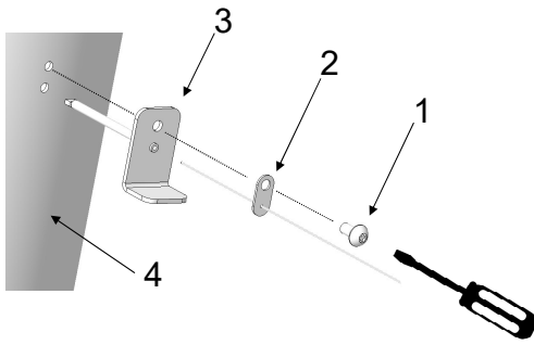
Fig. 42: Mounting the temperature sensor
