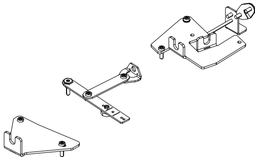
Fig. 39: Installation kit 363000
