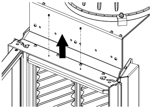
Fig. 74: Screwing out the bolts at the top
