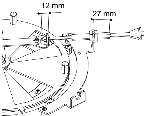
Fig. 50: Connecting the Bowden cable
