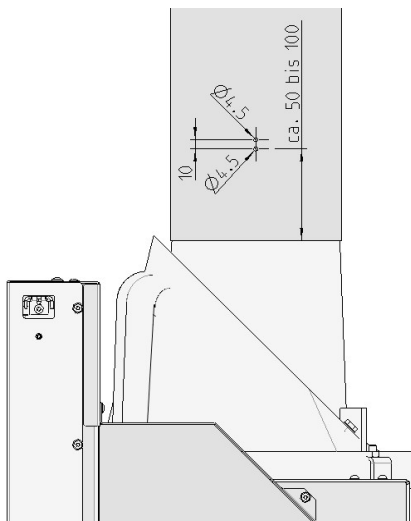
Fig. 41: Flue pipe drilling diagram
