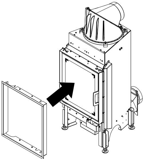
Fig. 76: Attaching the design frame
