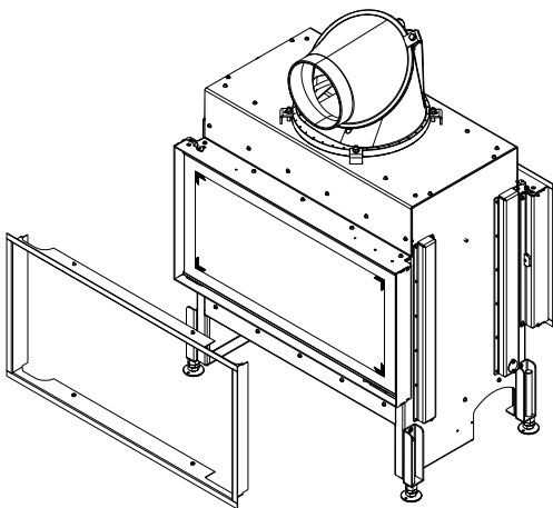
Fig. 84: Positioning the design frame on the back
