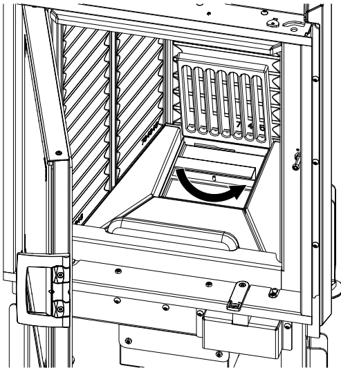
Fig. 98: Putting the cover on the ash box
