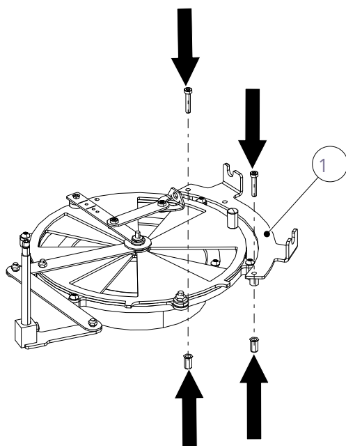
Fig. 47: Installing the installation kit
