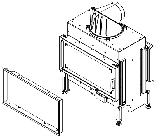
Fig. 81: Positioning the design frame
