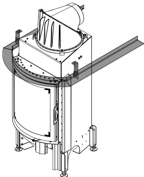
Fig. 89: Mounting the support frame
