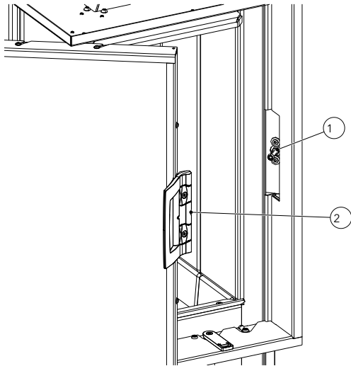
Fig. 92: Adjusting the door
