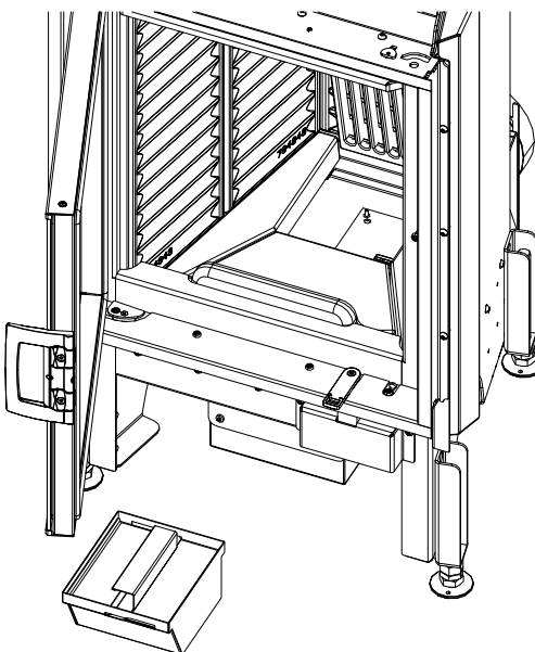
Fig. 100: Removing and emptying the ash box
