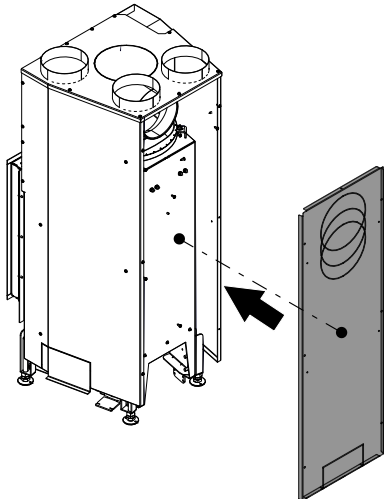
Fig. 63: Mounting the CV wall at the back
