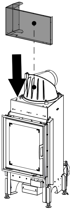
Fig. 59: Mounting the CV wall in front
