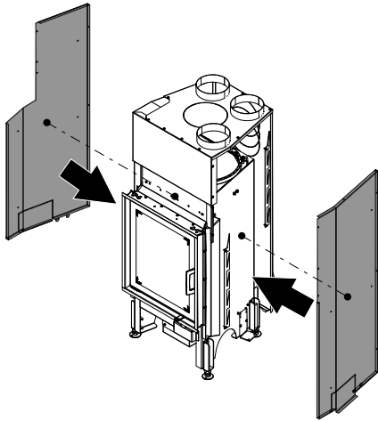
Fig. 61: Attaching CV wall right and left
