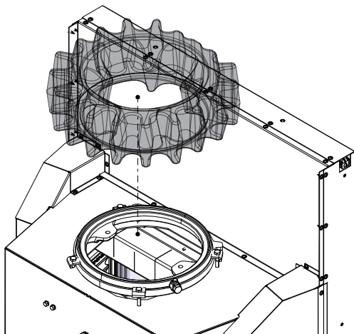
Fig. 31: Placing the top storage brick
