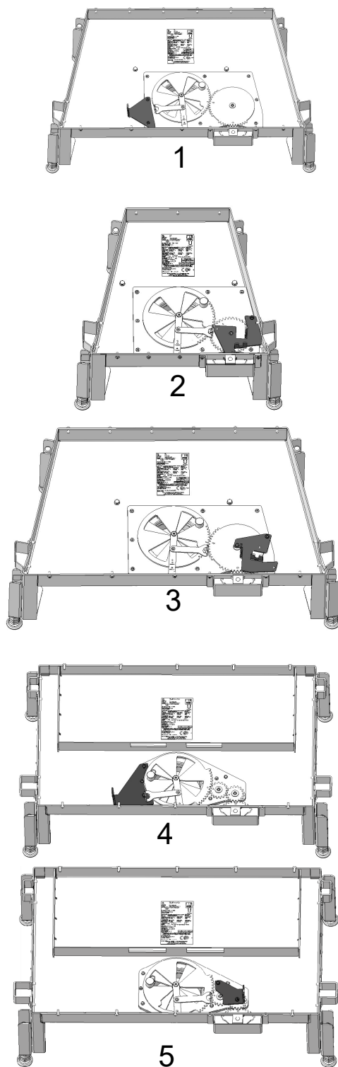
Fig. 44: Assembly situations
