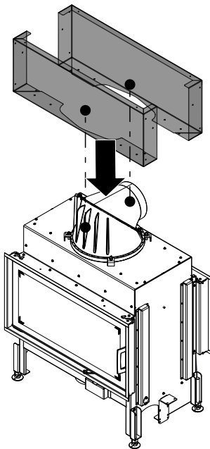
Fig. 68: Mounting CV wall at the top (front + rear)
