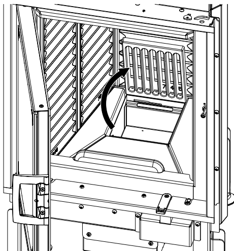
Fig. 97: Taking out or opening the grate
