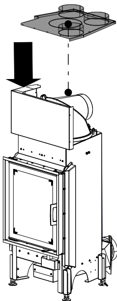
Fig. 60: Mounting the CV cover
