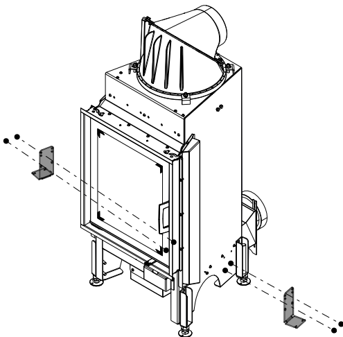
Fig. 55: Install mounting left and right
