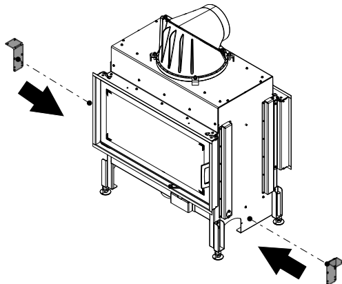
Fig. 65: Install mounting left and right
