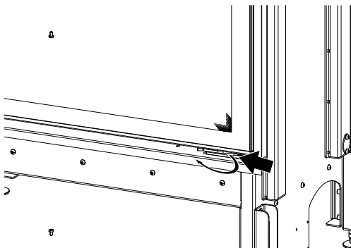
Fig. 85: Opening up the spring.
