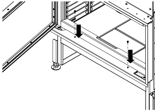
Fig. 87: Fixing the design frame at the bottom
