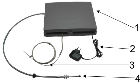
Fig. 38: Control unit
