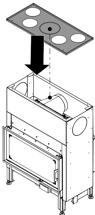
Fig. 71: Mounting the CV cover
