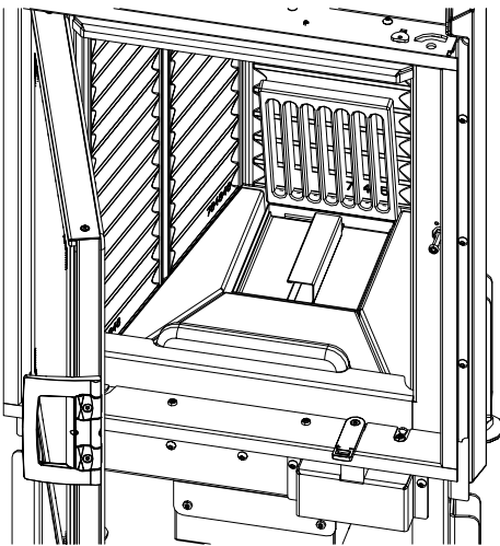
Fig. 99: Closing the cover
