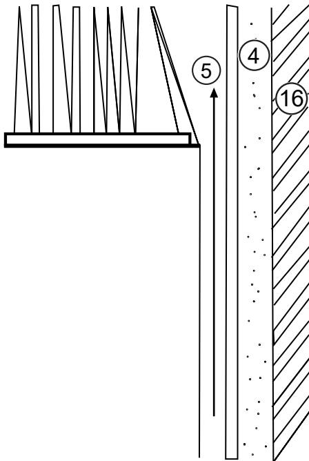
Fig. 7: Convection space
