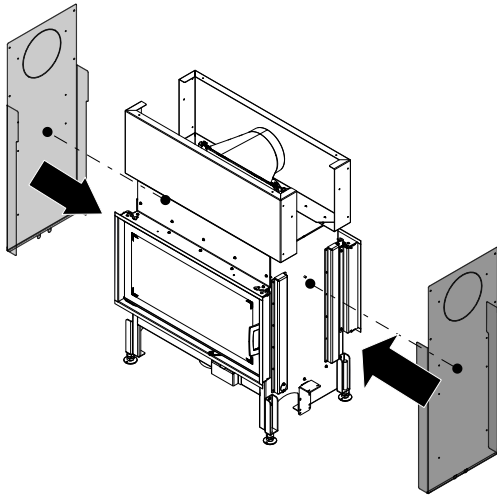
Fig. 69: Attaching CV wall left and right
