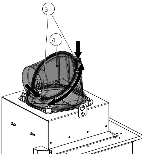
Fig. 94: Adjusting the smoke collector collar
