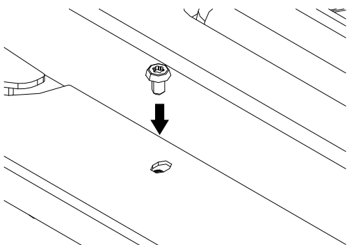
Fig. 77: Fastening the design frame
