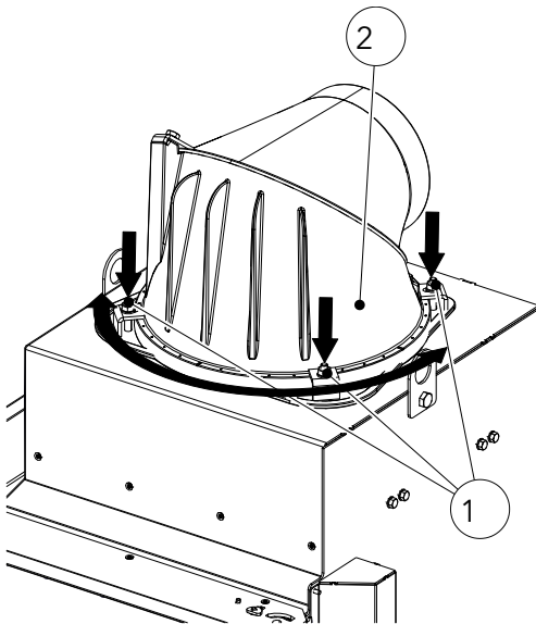
Fig. 93: Turning the smoke collector into the desired position
