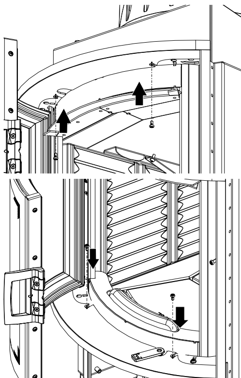
Fig. 80: Fixing the design frame
