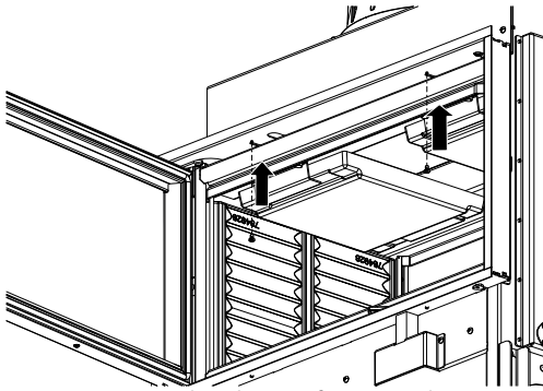
Fig. 82: Fixing the design frame at the top
