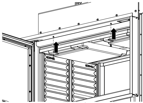
Fig. 86: Fixing the design frame at the top
