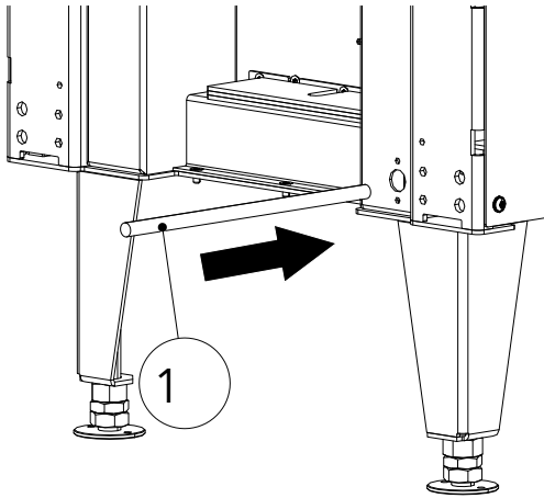
Fig. 49: Threading the Bowden cable
