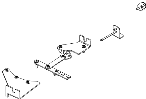
Fig. 40: Installation kit 363011
