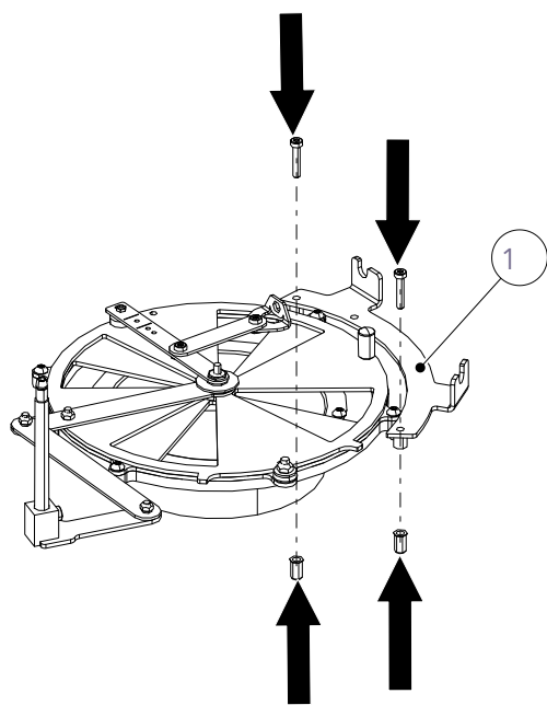
Fig. 13: Installing the installation kit
