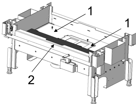
Fig. 12: Removing the parts
