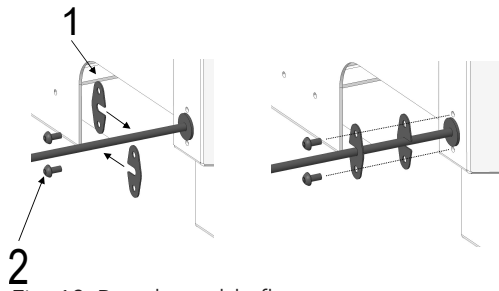
Fig. 18: Bowden cable flange
