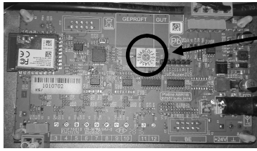
Fig. 20: Selecting the program
