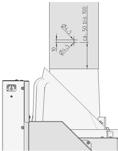
Fig. 7: Flue pipe drilling diagram
