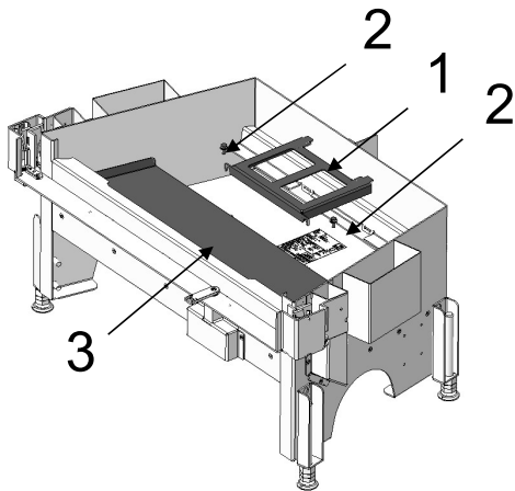
Fig. 11: Removing the parts
