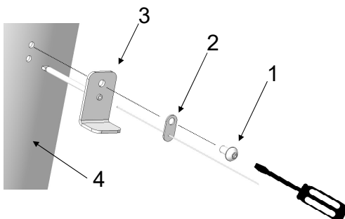
Fig. 8: Mounting the temperature sensor
