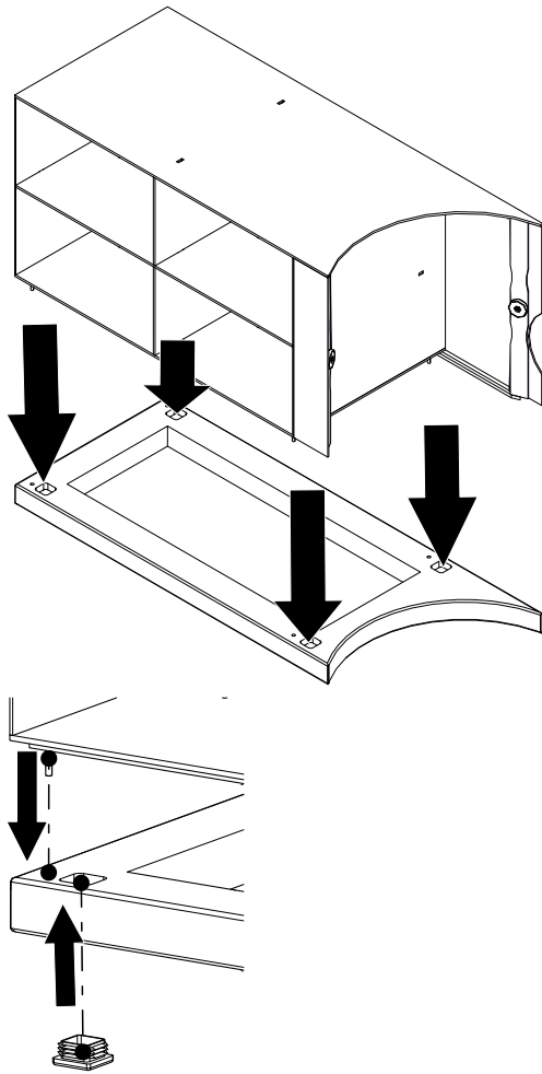
Fig. 1: Assembling the side box
