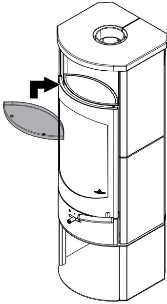
Fig. 1: Inserting the warming compartment.
